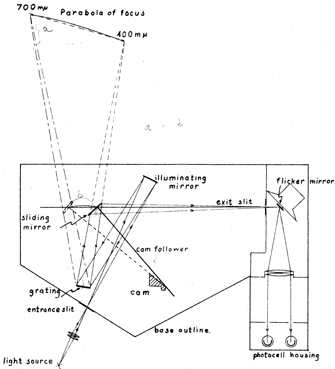
Figure 1. Optical System.
