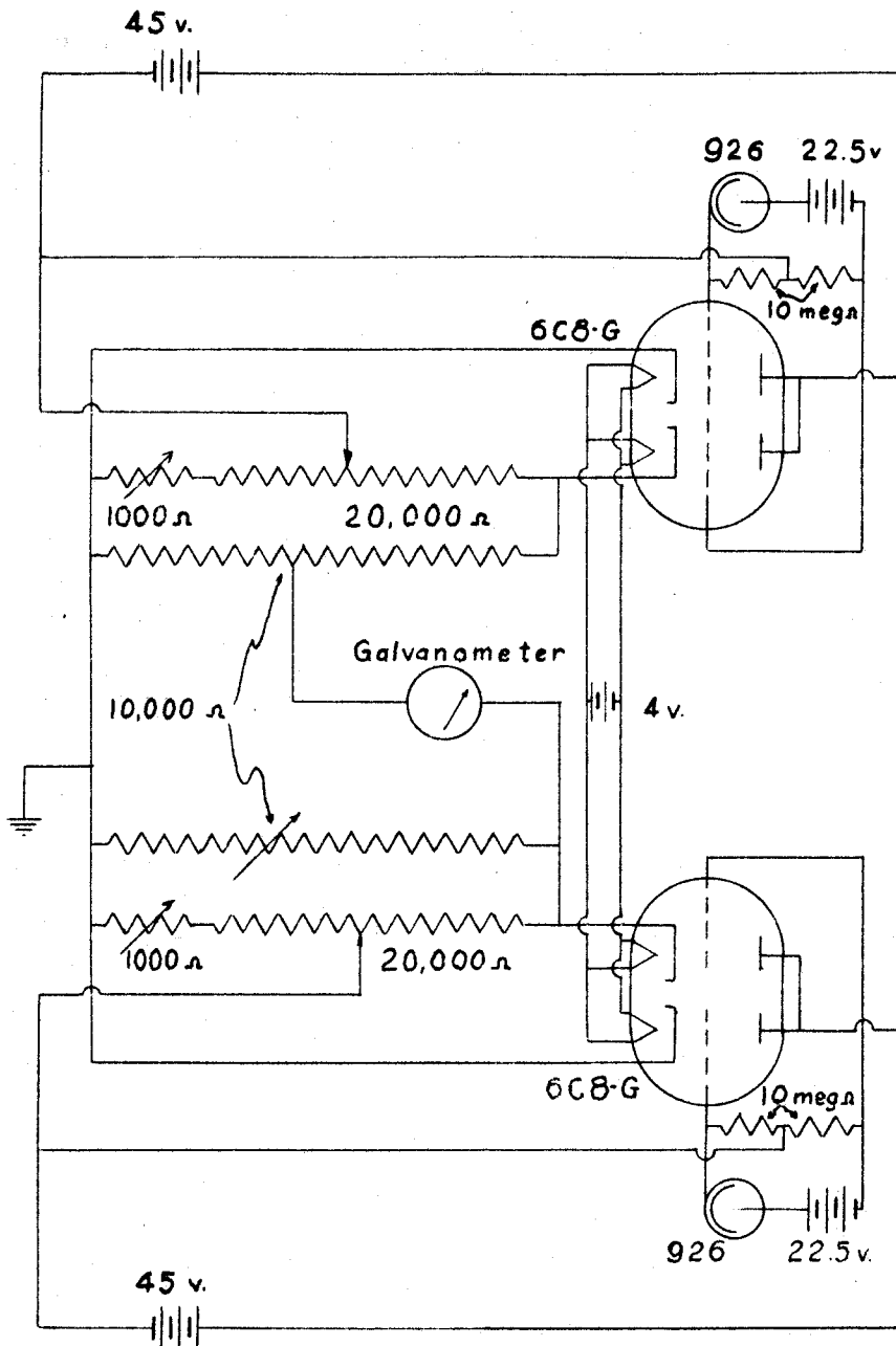
Figure 8. Final Amplifier Circuit.
