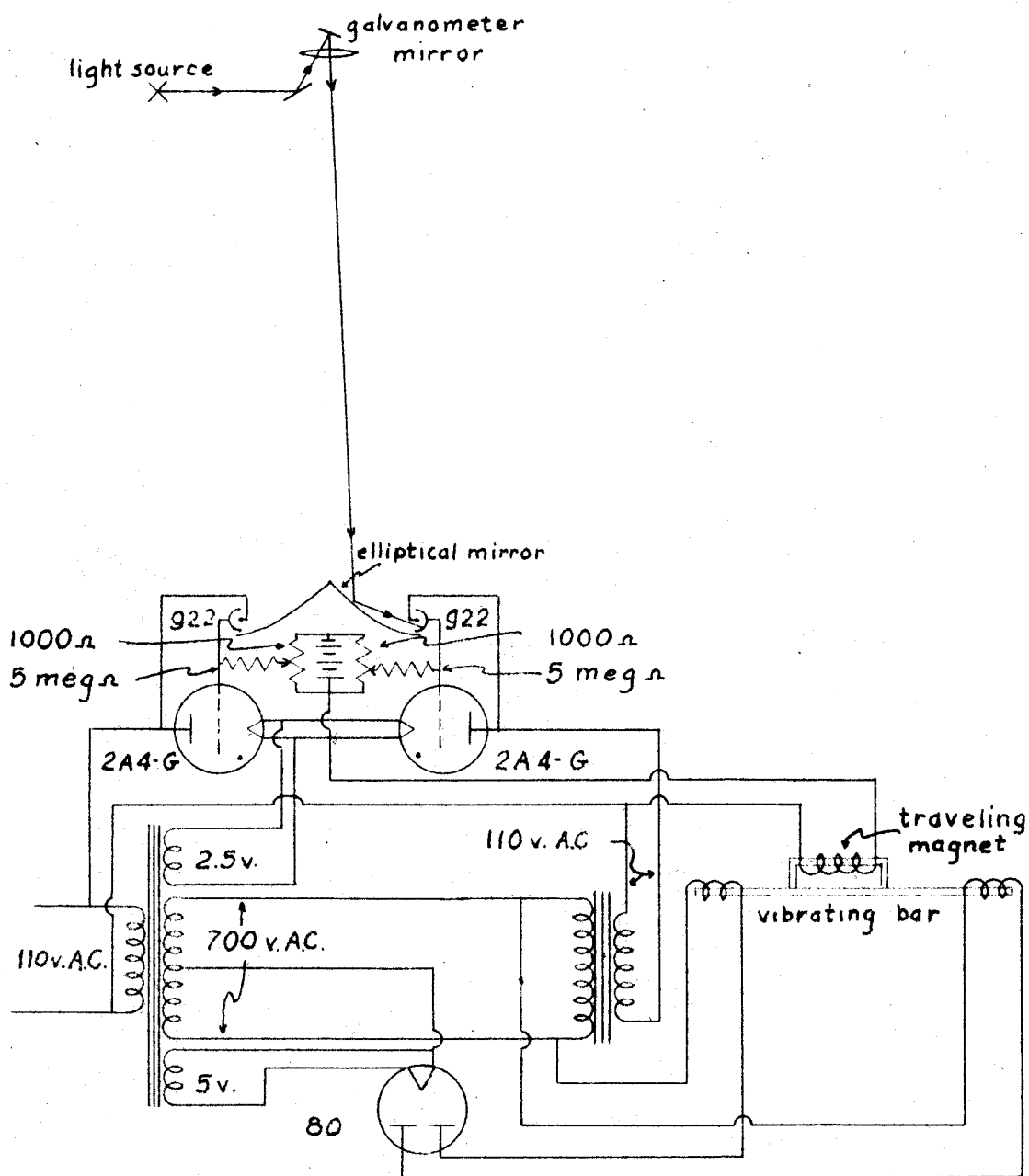
Figure 9. Recorder Circuit
