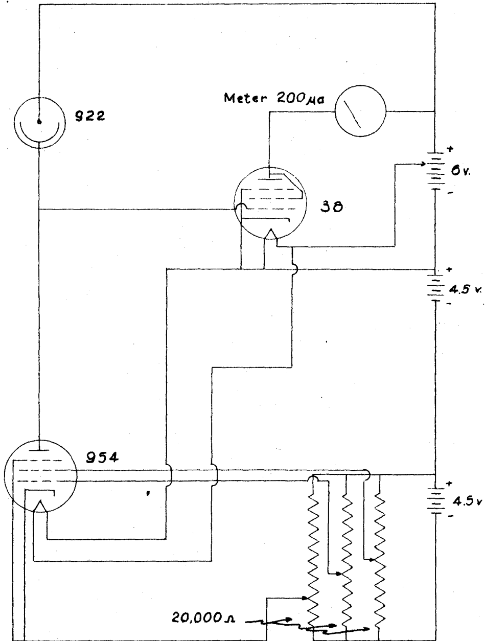
Figure 4. Shepard's Light Variation Indicator.
