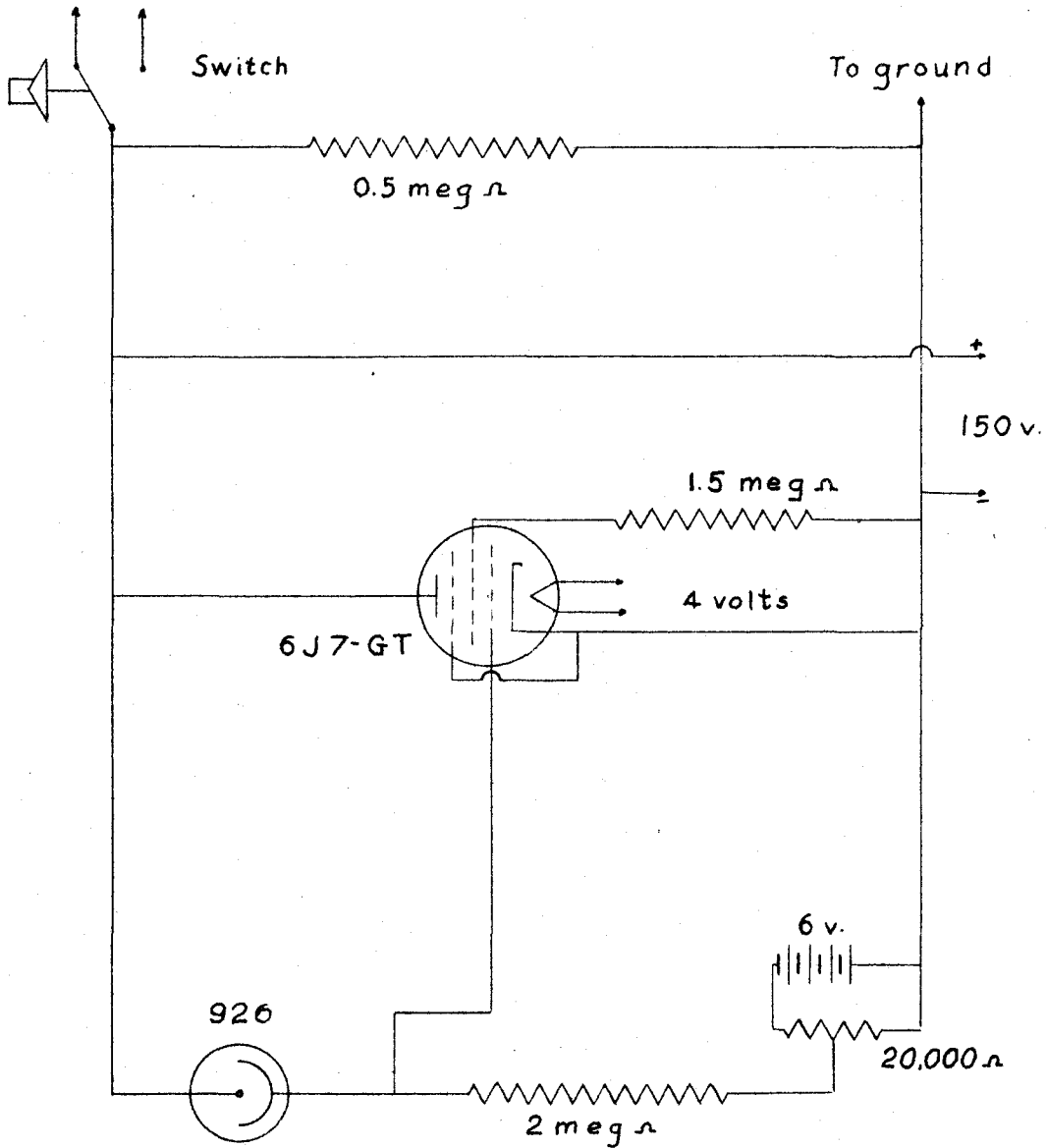
Figure 5. One Tube Pre-amplifier.
