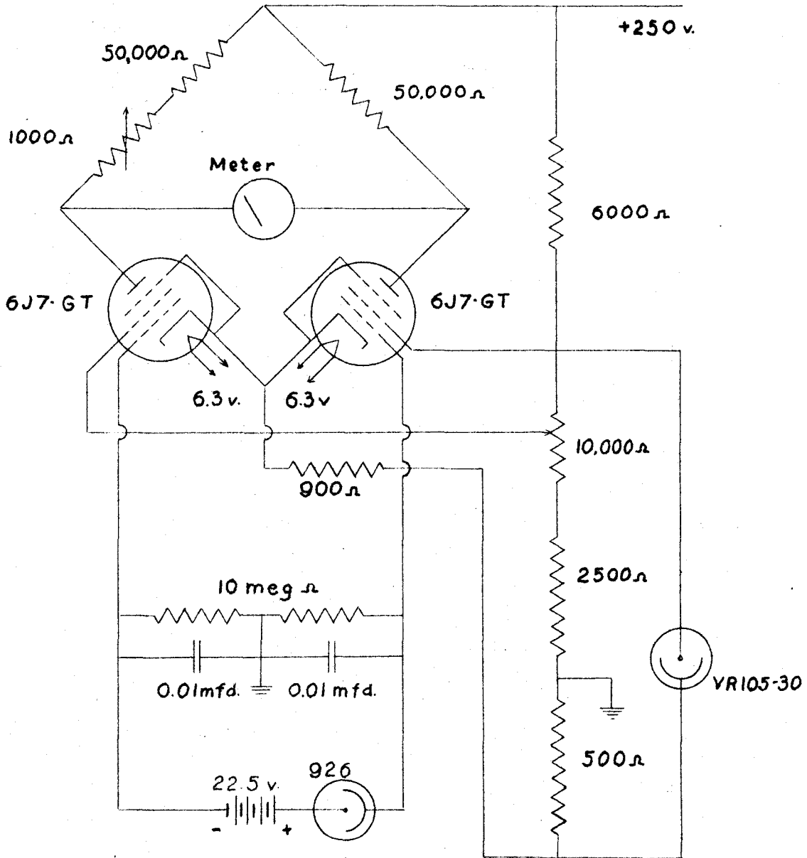
Figure 6. R.C.A. Bridge Amplifier.
